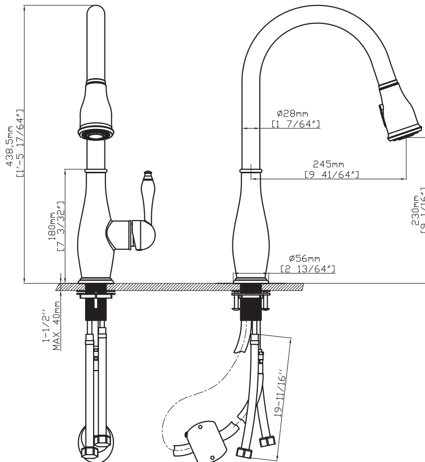
CRITICAL DIMENSIONS
